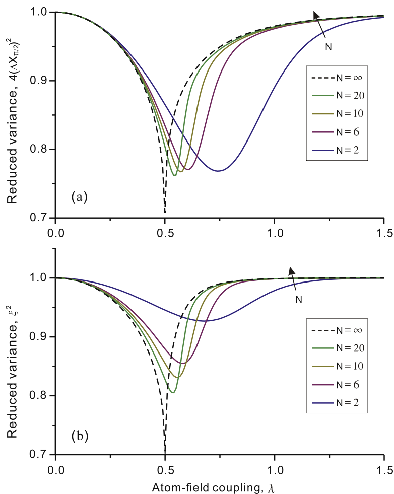
Figure 3. Degree of quadrature squeezing for the field mode 4(\Delta\hat{X}_{\pi/2})^2 (a), and that of spin squeezing for the atoms \xi^2 (b) against the coupling strength \lambda for the number of atoms N = 2, 6, 10, and 20 , as indicated by the arrow. Dashed lines: analytical results in the thermodynamic limit (i.e., N = \infty ). The local minimum of the reduced variances indicates quadrature squeezing of \hat{\rho}_{AB} at the critical point \lambda_{\text{cr}} = 0.5 (on resonance, as figure 1).
